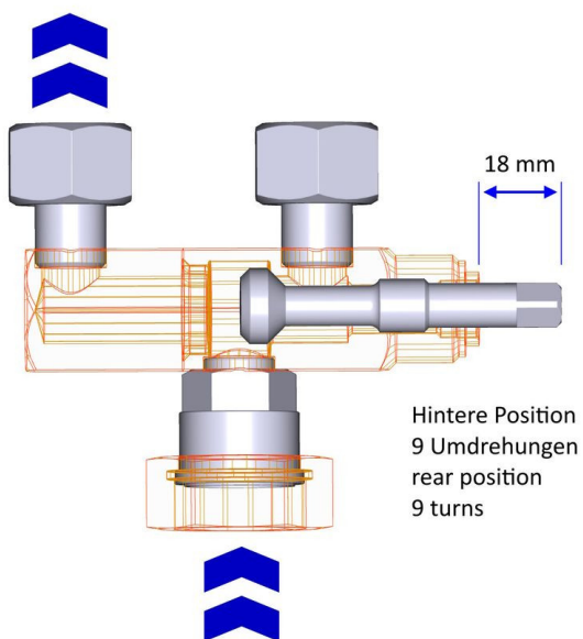
HANSA Wechselventil Einstellungen HANSA change-over (shuffle valve) setting
