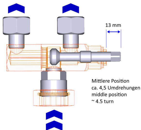
HANSA Wechselventil Einstellungen HANSA change-over (shuffle valve) setting
