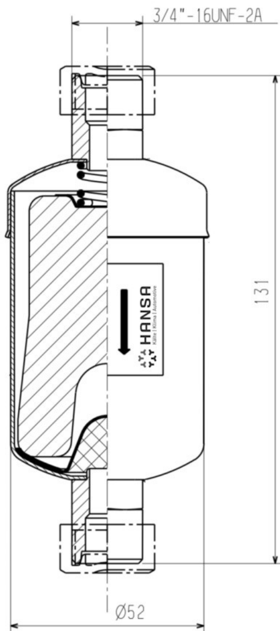
HANSA 2833612050
